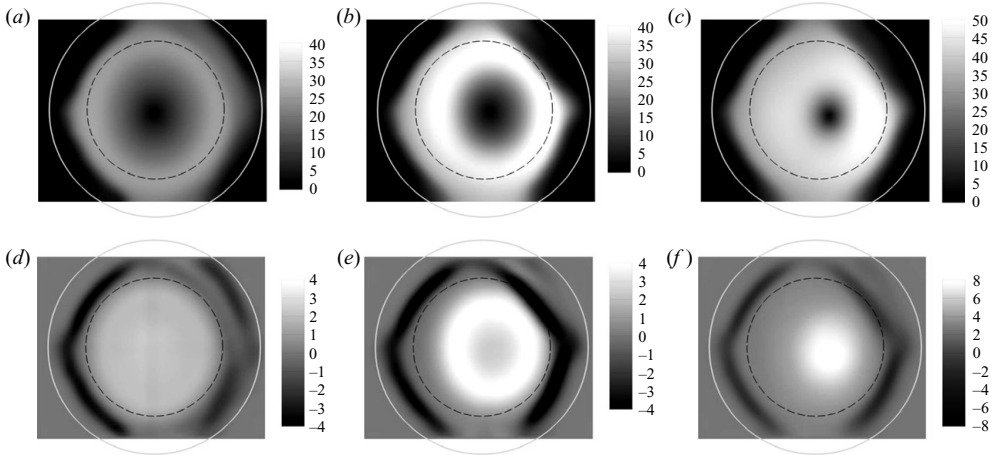
FIGURE 9. Average distributions of velocity magnitude in \text{mm s}^{-1} ( a–c ) and axial vorticity in \text{s}^{-1} ( d–f ) in three regimes with B_R = 0.68 mT: pure RMF flow ( a, d ); axial velocity reversal at F/Ta = 45 ( b, e ); swirl concentration at F/Ta = 140 ( c, f ). The outer circle displays the position of the container wall. The results may contain artefacts outside the inner dashed ring.
